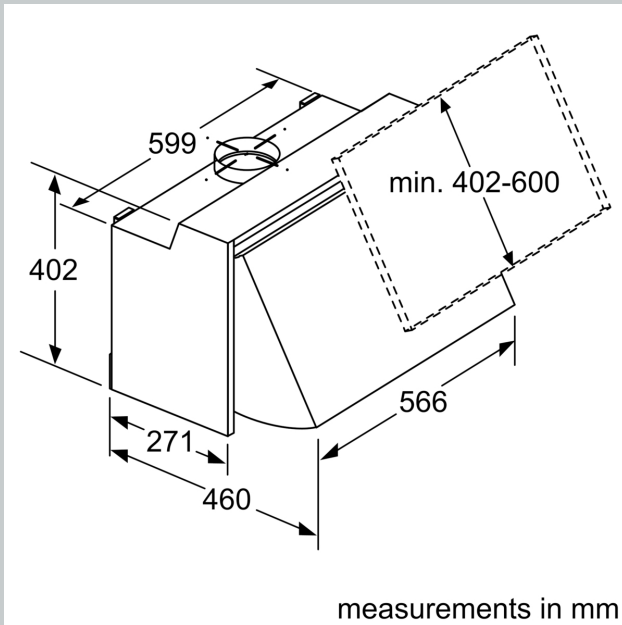
Dimensioned drawings
