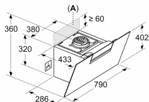
Measurements in mm Appliance in circulated air mode without duct
